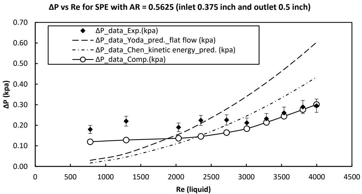
Figure 6.21. Single-phase flow pressure drop performance, compared with experimental data and other co-relations, \sigma_{exp} = 0.5625 , \dot{m}_l (kg/s) = 0.005 - 0.03
