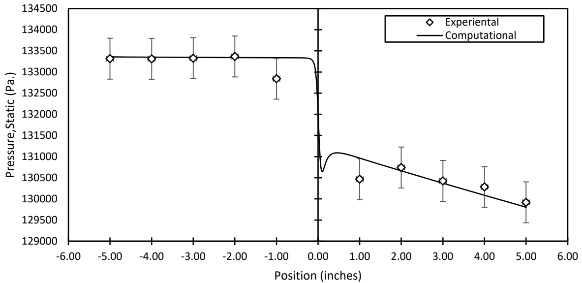
Pressure Profile, Comparison, Contraction AR-0.1444,0.03.kg/s
