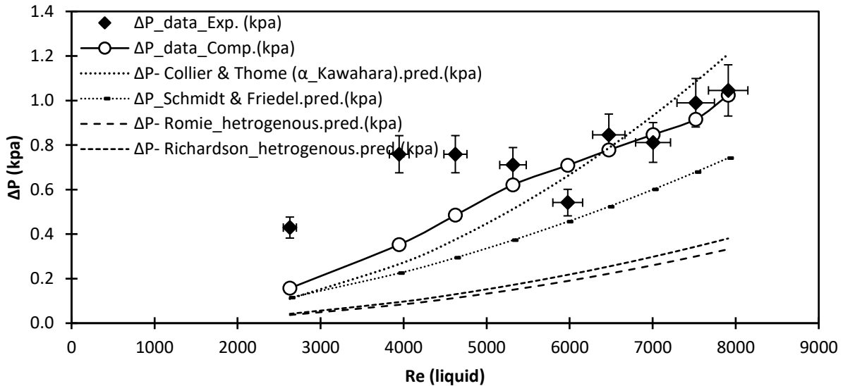
Two-Phase Expansion, \Delta P vs Re, comparison, \sigma = 0.1444 , All Flow Rates, Gas Flow Rate = 0.028.kg/s
