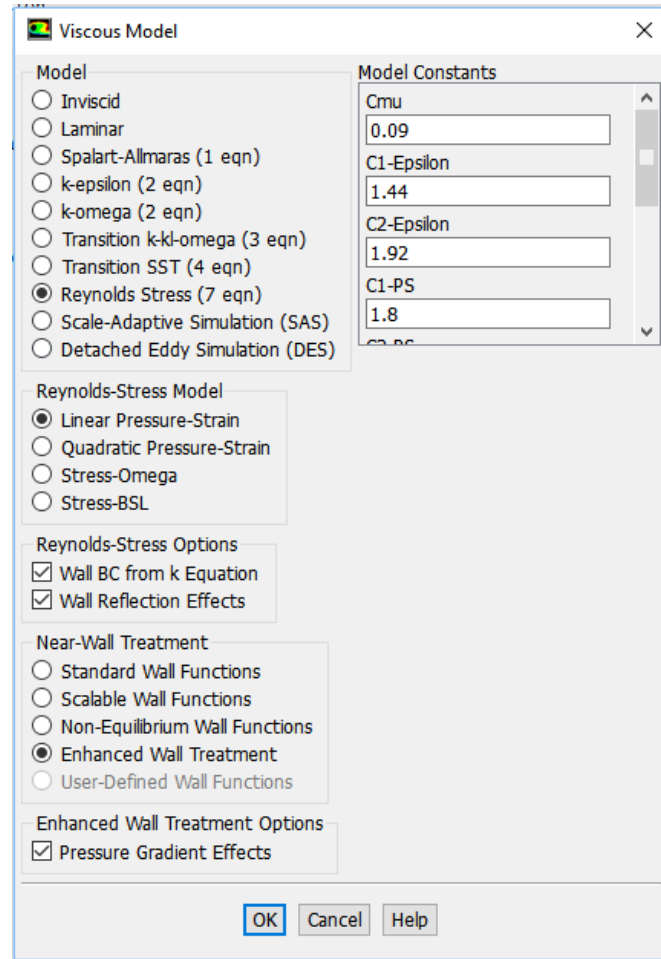
Figure 5.4. Model selection for single-phase flow where Reynolds Stress Model (5-equation) is shown
