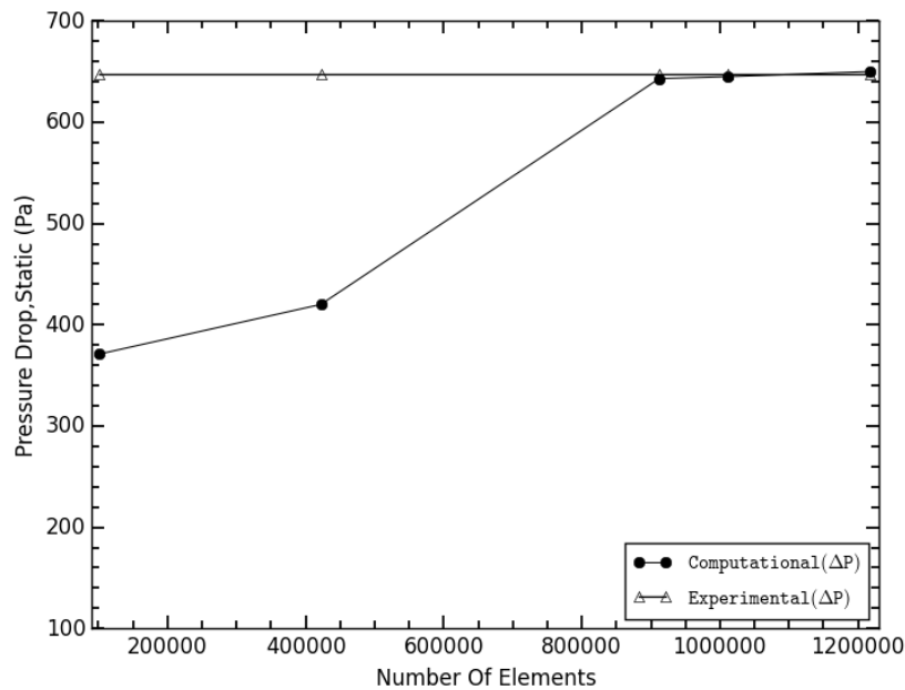
Figure 6.3. Pressure drop comparison for G.I.S. \sigma = 0.3844, m_g = 0.028 \frac{kg}{s}, m_l = 0.03 \frac{kg}{s}
