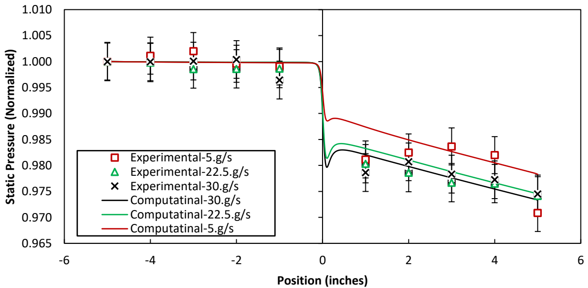
Single phase Contraction area ratio 0.1444 flow rates 5.g/s, 22.5.g/s, 30.g/s
